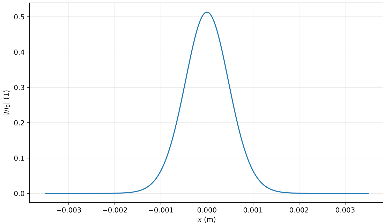
Intensity profile I(x, y = 0, z = 2.309m)/I_0 , P_{in}=0.2P_{cr} , artificial time
